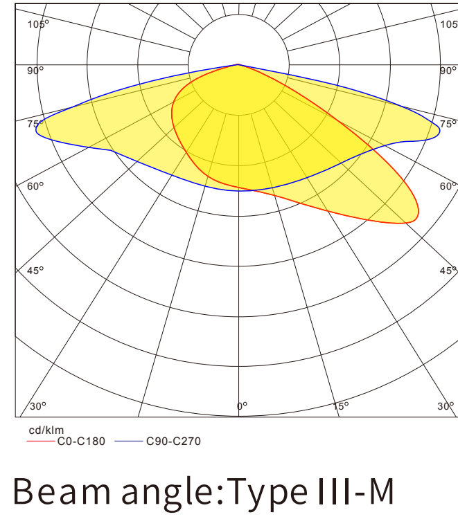
Beam angle: Type III-M
